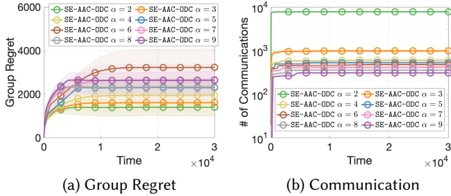
Fig. 10. Synchronous, 10 agents: 16 arms with Bernoulli rewards with average rewards uniformly randomly taken from Ad-Click [36], 10 agents all active in every time slots in time horizon T = 30\,000 . We report the number of communications and regrets averaged over 100 independent trials, and we plot the standard deviation as the shaded area.
