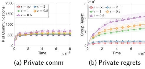
Fig. 6. Performance of SE-AAC-ODC-CTB
