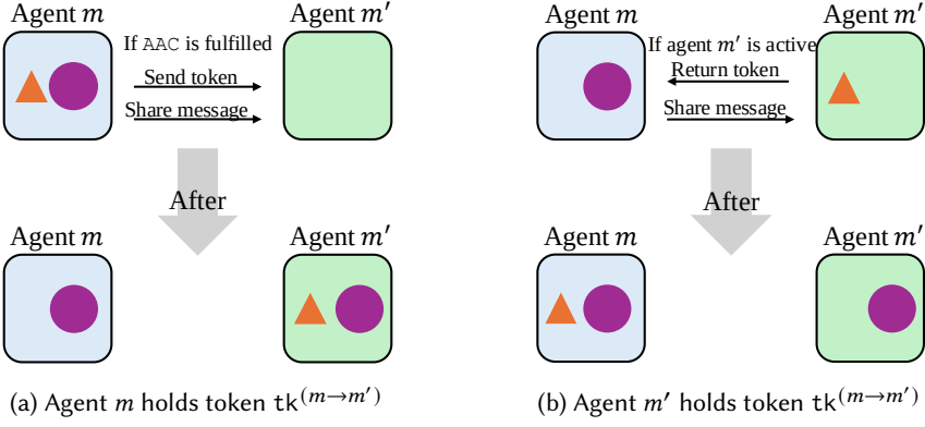
Fig. 2. Illustration of the token-based ODC mechanism: ▲ Token tk^{(m \rightarrow m')} ● Message to share
