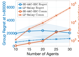
(a) Increase Agents
