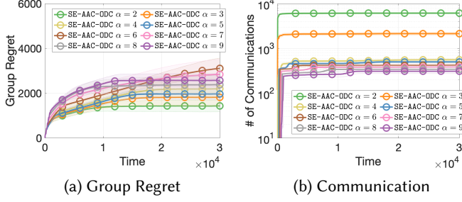
Fig. 8. Asynchronous, 10 agents: 16 arms with Bernoulli rewards with average rewards uniformly randomly taken from Ad-Click [36], 10 agents with activation frequency of agent m follows a sine function, \sin(\theta_m + t/30) , where the phase shifts \theta_m = m/5 , m \in \{1, \dots, M\} differ for different agents. We report the number of communications and regrets after T = 30\,000 time slots averaged over 100 independent trials, and we plot the standard deviation as the shaded area.
