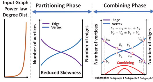
Fig. 7. Main idea of BPart with two-phase partition.
