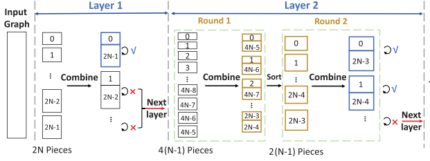
Fig. 9. Multi-layer combination strategy.
