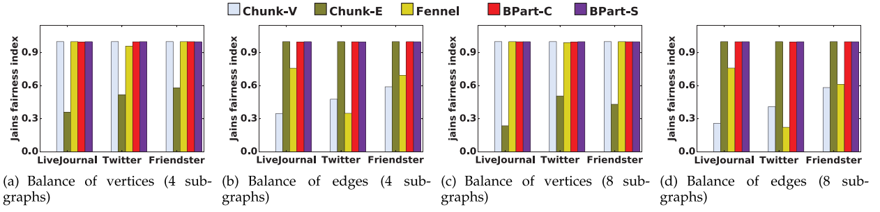
Fig. 12. Balanced degree estimated with Jain's fairness index: (a) and (b) show the balance trade-off when partitioning to 4 subgraphs, and (c) and (d) show the trade-off when partitioning to 8 subgraphs.
