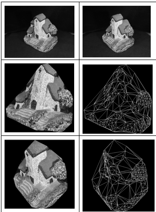
Figure 2: Results for the reconstruction of a model house. The first row contains the first and last (15 th ) image of the input sequence. The second and third rows contain two reconstructed textured views and their wire-frames.
