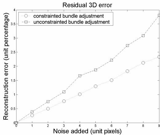
Fig 1. Comparison between the residual 3D errors of the methods
