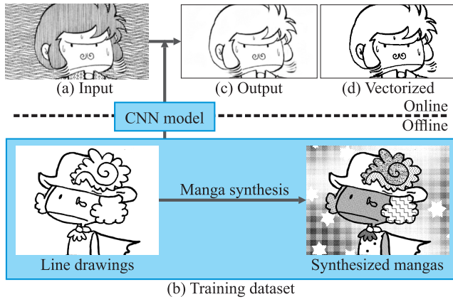
Fig. 5. System overview. ©Minamoto Tarou
