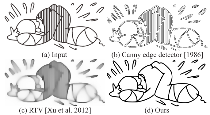
Fig. 4. Comparison of existing line extraction methods.
