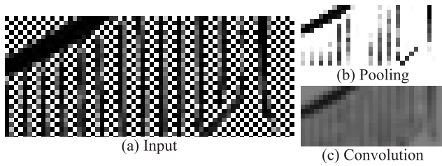
Fig. 11. Downsampling by different methods. (b) Max-pooling breaks the spatial continuity. (c) Convolution achieves better downsampling results.
