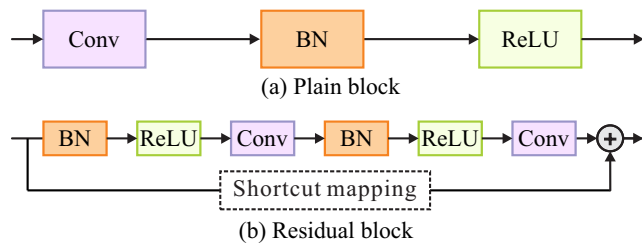
Fig. 10. Plain block structure vs. residual block structure.
