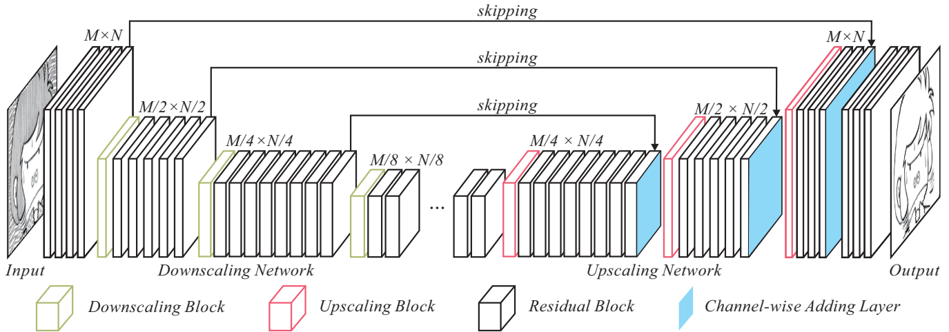
Fig. 9. Overall structure of the proposed network. ©Minamoto Tarou
